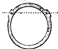
SECTION OF DOULTON'S LIDDED DRAIN-TUBES.
