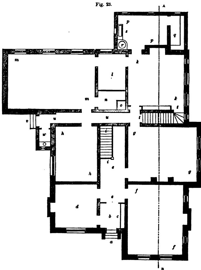
GROUND-PLAN OF FARMHOUSE—SCALE IN PLATE XVIII.
