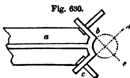
Fig. 630. JUNCTION OF FOUR GIRDEES ON CAP OF COLUMN—SCALE, \frac{1}{2} INCH TO THE FOOT.
