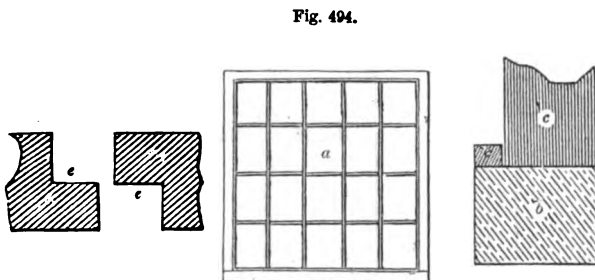
DETAILS OF SLIDING WINDOW.
