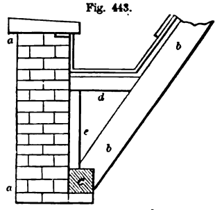
BRIDGED GUTTER—SCALE, \frac{1}{2} INCH TO THE FOOT.
