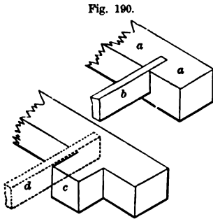
GOOD AND BAD METHODS OF SETTING FLOORING-JOISTS—SCALE, \frac{1}{4} INCH TO THE FOOT.
