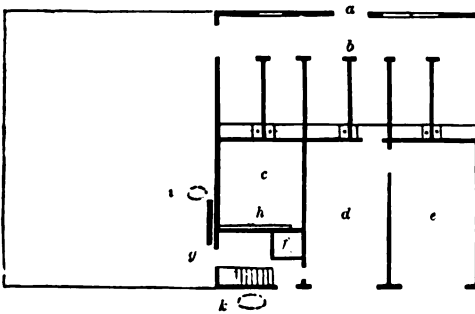
PLAN OF WESTERN STATES AMERICAN FARM-BUILDINGS.
