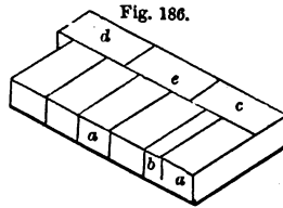
Fig. 186. PLAN OF SECOND COURSE OF 8-INCH WALL —SCALE, 1/2 INCH TO THE FOOT.
