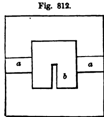
PLAN OF SHOE FOR RECEIVING ENDS OF GIRDER—SCALE, 1 INCH TO THE FOOT.
