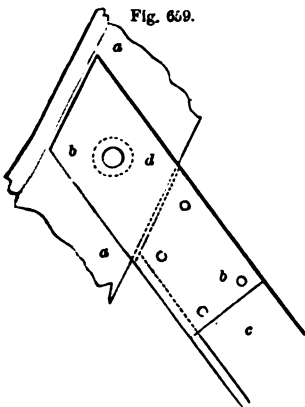
JOINING OF UPPER END OF STRUT WITH RAFTER.
