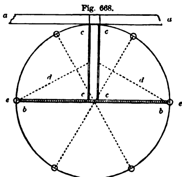
Fig. 668. PLAN OF HORSE-WALK FOR THRASHING-MILL.—SCALE, ¼ INCH TO THE FOOT.
