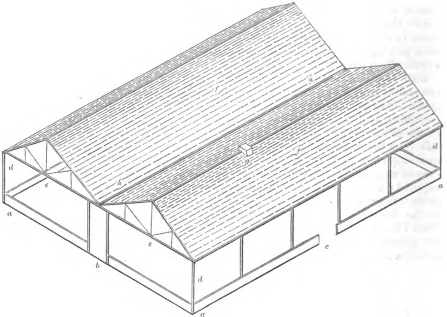
ISOMETRICAL PERSPECTIVE OF A COVERED STACKYARD
