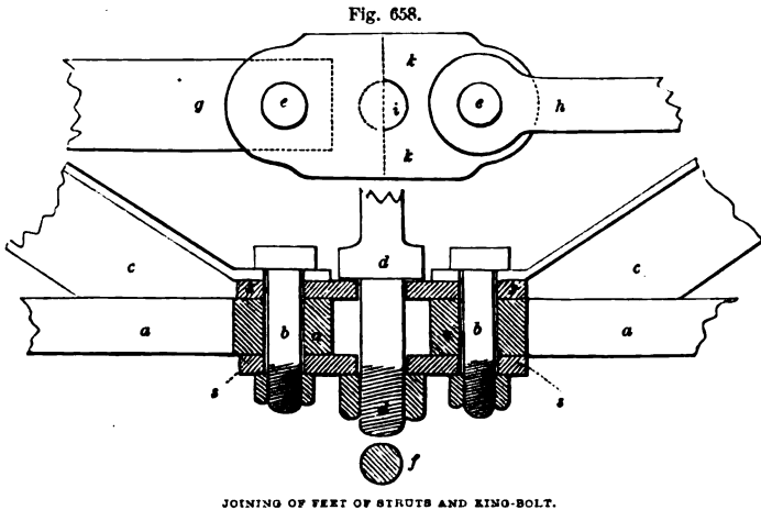
JOINING OF FEET OF STRUTS AND KING-BOLT.
