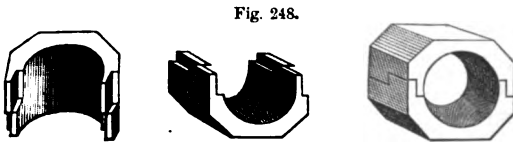
FIG. 248. PERSPECTIVE VIEWS OF SADDLES FOR COOPER'S LIPPED DRAIN-TUBES.
