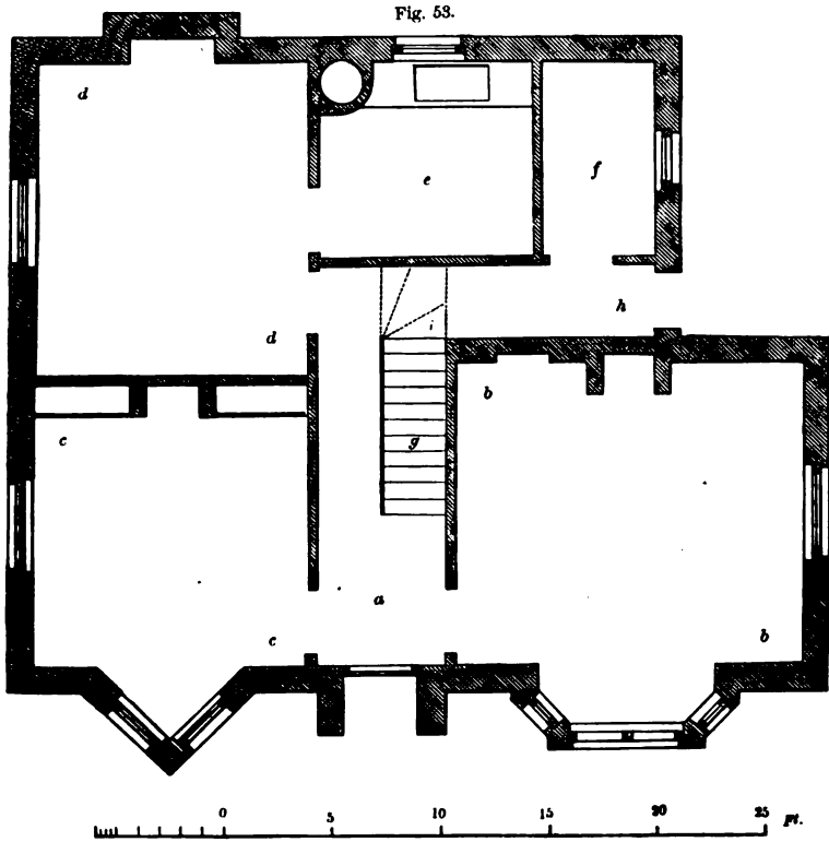
GROUND-PLAN OF A SECOND-CLASS FARMHOUSE.
