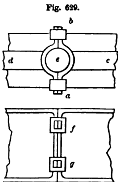
Fig. 629. JUNCTION OF GIRDEES—SCALE, \frac{1}{2} INCH TO THE FOOT.
