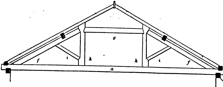
QUEEN-POST ROOF—SCALE, \frac{1}{4} INCH TO THE FOOT.
