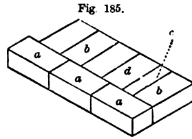
Fig. 185. PLAN OF FIRST COURSE OF 8-INCH WALL IN OLD ENGLISH BOND—SCALE, 1/2 INCH TO THE FOOT.
