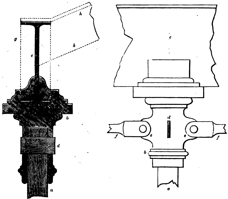
SECTION AND ELEVATION OF WROUGHT-IRON COLUMNS FOR SHEDS.
