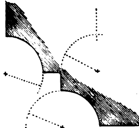
MOULDINGS OF JAMB AND MULLION OF DOORWAY—SCALE, \frac{1}{2} FULL SIZE.
