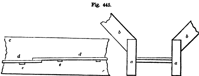
SECTION AND ELEVATION OF VALLEY-GUTTER—SCALE, \frac{1}{2} INCH TO THE FOOT.
