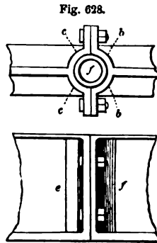
JUNCTION OF GIRDERS WITH CIRCULAR NECK TO COLUMNS—SCALE, 1/2 INCH TO THE FOOT.
