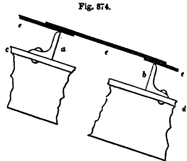
FIXING OF SLATES WITH IRON ROOF—SCALE IN FIG. 857.
