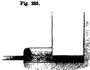
SECTION OF FIRECLAY HEARTH.
