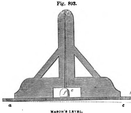
MASON'S LEVEL.
