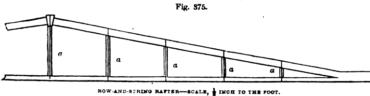
BOW-AND-STRING RAFTER—SCALE, 1/4 INCH TO THE FOOT.
