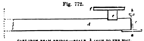
CAST-IRON BEAM BRIDGE—SCALE, 1/4 INCH TO THE FOOT.
