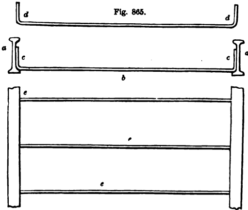
PLAN AND ELEVATION OF FIREPROOF FLOORING—SCALE, 1/2 INCH TO THE FOOT.
