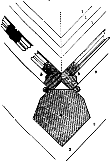
PART SECTIONAL PLAN OF V WINDOW—SCALE, 1 INCH TO THE FOOT.
