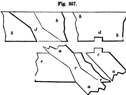
JOINING OF TIMBERS AT RIGHT ANGLES—SCALE, 1 INCH TO THE FOOT.
