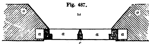
PLAN OF FIXED WINDOW.
