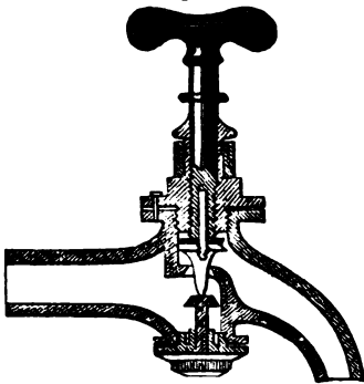
CHRIMES'S WATER-TAP.
