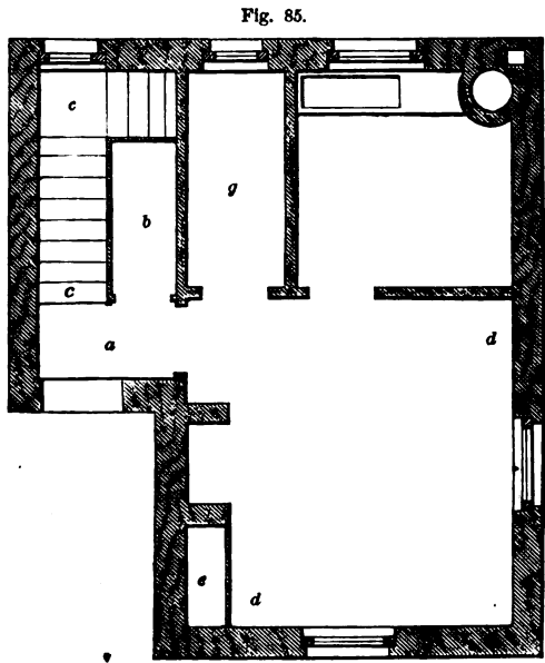
GROUND-PLAN OF A TWO-STOREYED DETACHED COTTAGE—SCALE IN FIG. 75.
