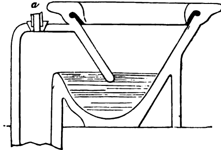
EARTHENWARE CLOSET-PAN WITH TRAP
