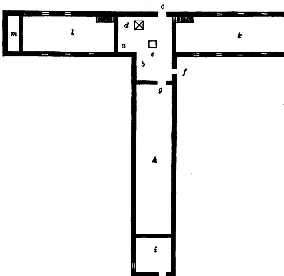
UPPER STOREY OF A STEADING FOR MIXED HUSBANDRY.
