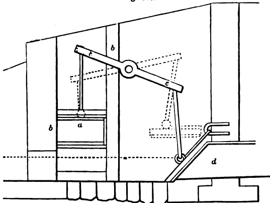
LONGITUDINAL SECTION OF SELF-ACTING SLUICE.
