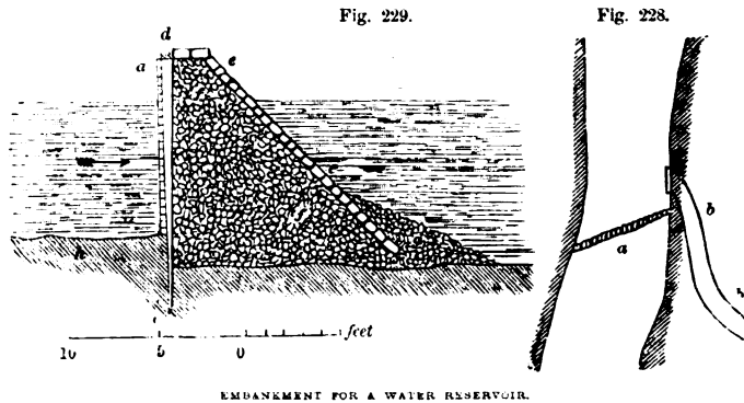
EMBANKMENT FOR A WATER RESERVOIR.
