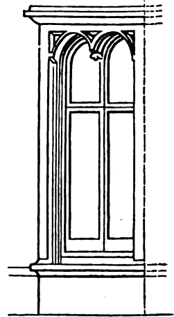
SIDE ELEVATION OF WINDOW IN FIG. 50. SCALE, 1 INCH TO THE FOOT.
