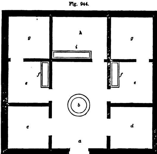
PLAN OF DETACHED PIGGERY—SCALE, 1/2 INCH TO THE FOOT.
