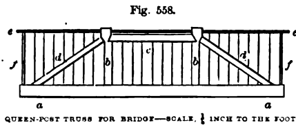
QUEEN-POST TRUSS FOR BRIDGE—SCALE, \frac{1}{4} INCH TO THE FOOT.
