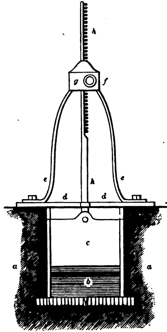
ELEVATION OF IRON SLUICE VALVE AND RACK—SCALE. 1/2 INCH TO THE FOOT.
