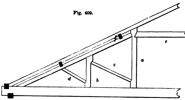
TRUSS WITH TWO QUEEN-POSTS FOR 47-FOOT SPAN—SCALE, \frac{1}{4} INCH TO THE FOOT.
