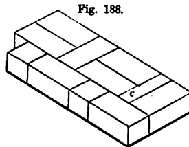
Fig. 188. PLAN OF SECOND COURSE OF 8-INCH WALL, FLEMISH BOND—SCALE, 1/2 INCH TO THE FOOT
