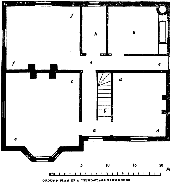
GROUND-PLAN OF A THIRD-CLASS FARMHOUSE.
