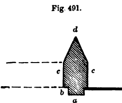
ASTRAGALS OF SASH WINDOW.
