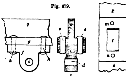
RIVETING STRUTS TO RAFTERS.
