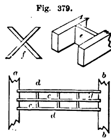
TRUSSING OF FLOORING BEAMS—SCALE, 1/4 INCH TO THE FOOT.
