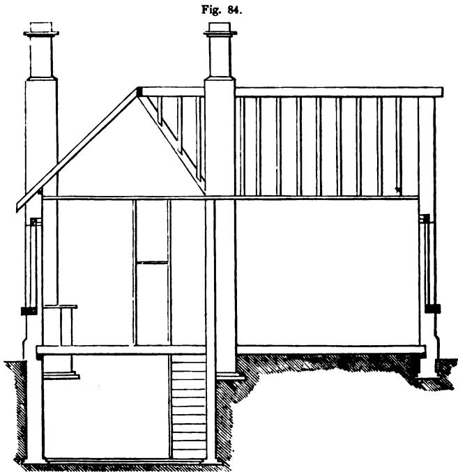
VERTICAL SECTION OF A SINGLE-STORYED DETACHED COTTAGE—SCALE IN FIG. 81.
