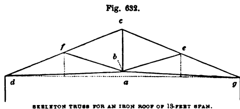
Fig. 632. SKELETON TRUSS FOR AN IRON ROOF OF 18-FOOT SPAN.
