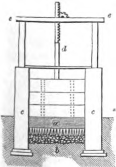
WOODEN SLUICE IN STONE GROOVES.
