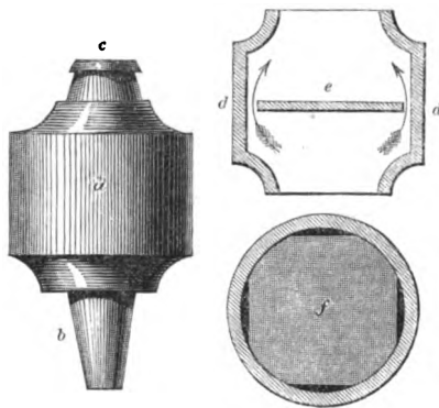
GAS REGULATOR.
