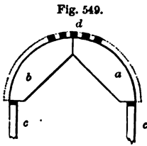
Fig. 549. CENTRE FOR A DOOR ARCH— SCALE, \frac{1}{4} INCH TO THE FOOT.
