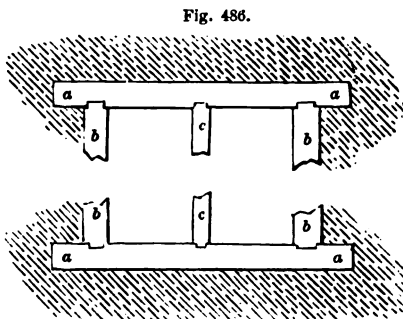
PLAN OF FRAMING FOR A FIXED WINDOW.
