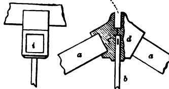
SHOES FOR RING-BOLT HEADS—SCALE, \frac{1}{2} INCH TO THE FOOT.
