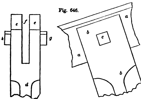
UPPER END OF CAST-IRON STRUT.
