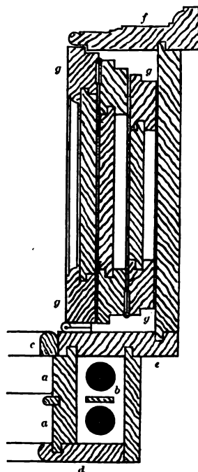
SASH-WINDOW.
