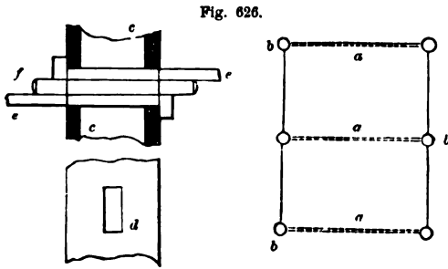
POSITION AND FIXING OF TIE-RODS—SCALE, 1 INCH TO THE FOOT.
