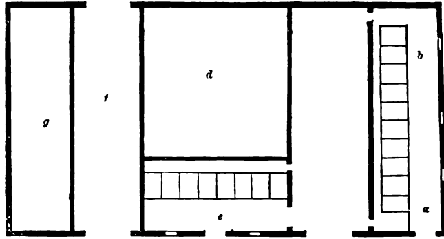
PLAN OF DUTCH BARN—SCALE AS IN FIG. 965.
