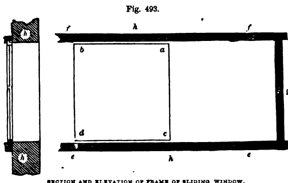
SECTION AND ELEVATION OF FRAME OF SLIDING WINDOW.
