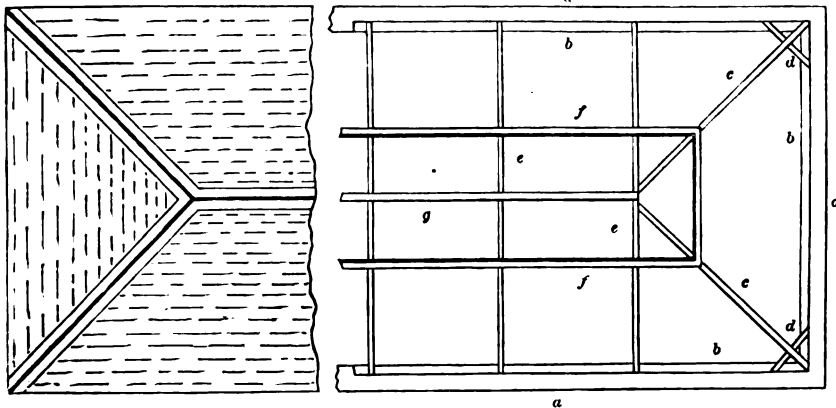
PLAN OF HIPPED-ROOF.
