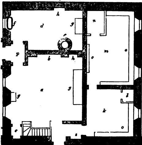
GROUND-PLAN OF A KITCHEN, ETC., OF FARMHOUSE.
