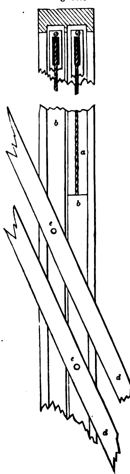
LONGITUDINAL SECTION OF SHAW'S PATENT WINDOW.
