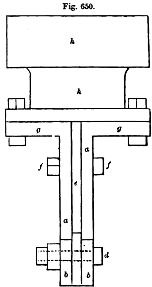
SIDE ELEVATION OF FIG. 649.
