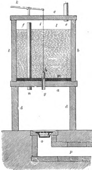
A RAIN-WATER CISTERNS.
