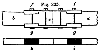
Fig. 325. JOINING TIMBERS IN THE DIRECTION OF THEIR LENGTH—SCALE, ¼ INCH TO THE FOOT.
