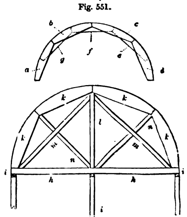
Fig. 551. CENTRES FOR STONE CIRCULAR ARCHES—SCALE, \frac{1}{4} INCH TO THE FOOT.
