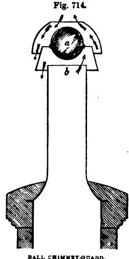
BALL CHIMNEY-GUARD.
