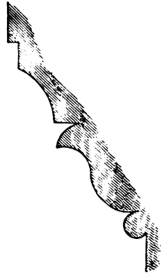
SUMMER-STONE—SCALE, \frac{1}{2} FULL SIZE.
