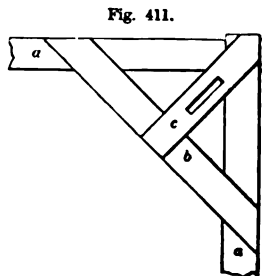
DRAGON-PIECE AND DRAGONAL TIE TO SUPPORT HIP-RAFTERS.
