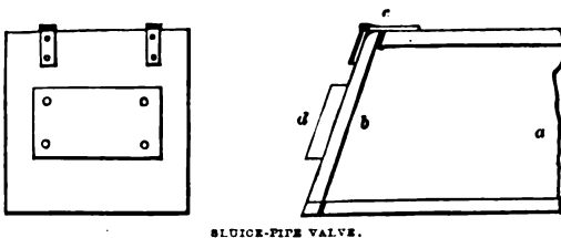
SLUICE-PIPE VALVE.
