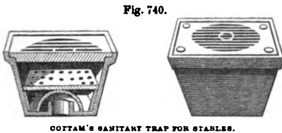
COTTAM'S SANITARY TRAP FOR STABLES.
