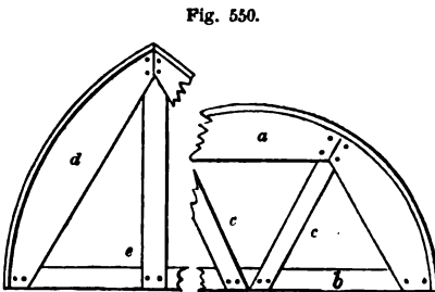
Fig. 550. CENTERINGS FOR GOTHIC AND SEMICIRCULAR ARCHES— SCALE, \frac{1}{4} INCH TO THE FOOT.
