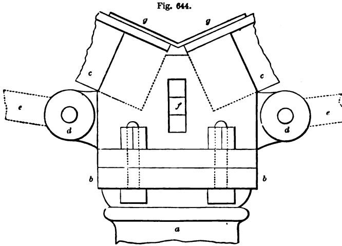
HAFTER-SHOES FOR ROOF IN FIG. 613—SCALE IN FIG. 637.
