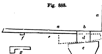
PLAN OF PART OF JOINER'S BENCH.
