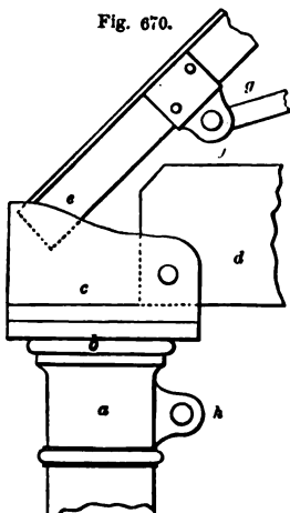
Fig. 670. SHOE FOR FEET OF RAFTERS, TIE-BEAM, AND TIE-NODS.—SCALE, 1 INCH TO THE FOOT.
