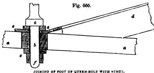
JOINING OF FOOT OF QUEEN-BOLT WITH STRUT.
