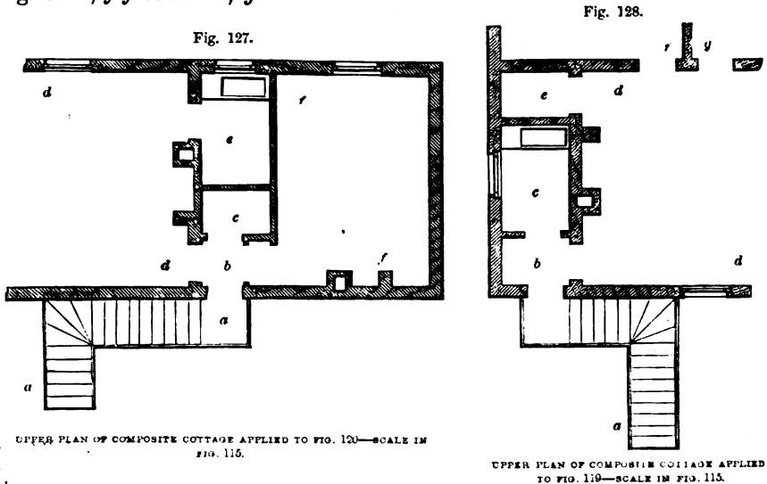
UPPER PLAN OF COMPOSITE COTTAGE APPLIED TO FIG. 119—SCALE IN FIG. 115.
