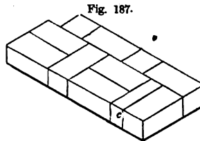
Fig. 187. PLAN OF FIRST COURSE OF 8-INCH WALL IN FLEMISH BOND—SCALE, 1/2 INCH TO THE FOOT
