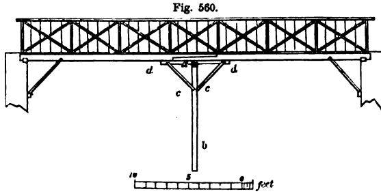
ELEVATION OF BRIDGE OF 32-FOOT SPAN.
