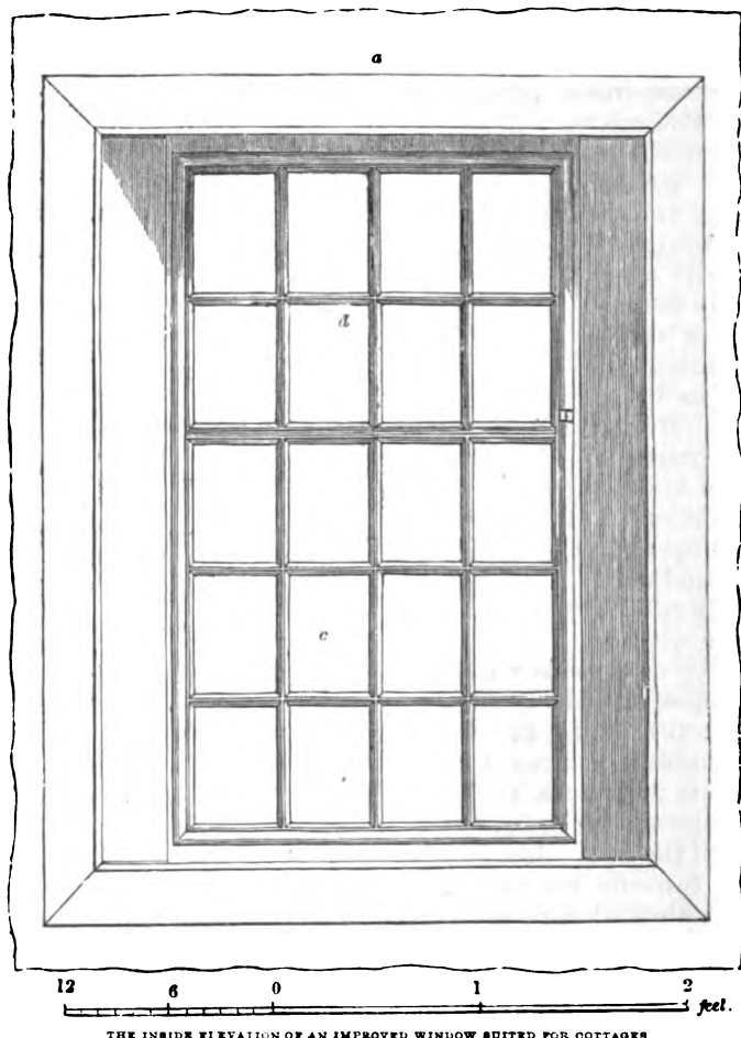
THE INSIDE ELEVATION OF AN IMPROVED WINDOW SUITED FOR COTTAGES.
