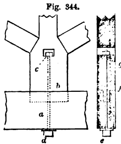
CONNECTION OF KING-POST WITH TIE-BEAM, WITH BOLT—SCALE, 1/2 INCH TO THE FOOT.
