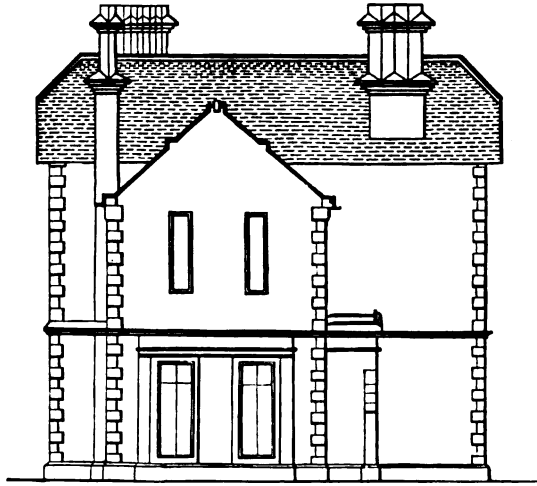
END ELEVATION OF TUDOR HOUSE—SCALE IN FIG. 41.
