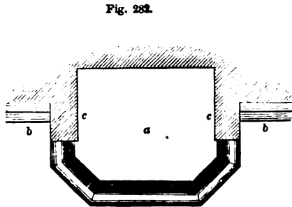
PLAN OF FIRECLAY HEARTH
