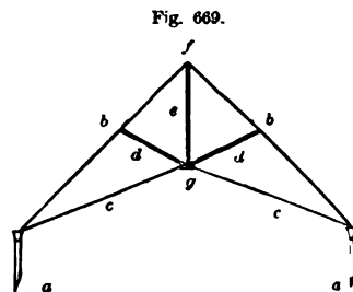
Fig. 669. SKELETON TRUSS FOR THRASHING-MILL.— SCALE, ¼ INCH TO THE FOOT.
