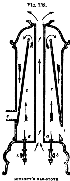
RICKETT'S GAS-STOVE.
