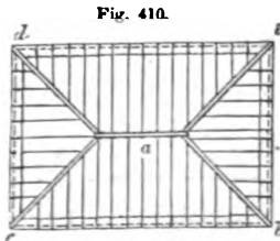
ROOF WITH HIP-RAFTER—SCALE, \frac{1}{4} INCH TO THE FOOT.
