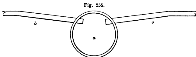
SECTION OF CROSS-CULVERT AND UNDER-DRAINS
