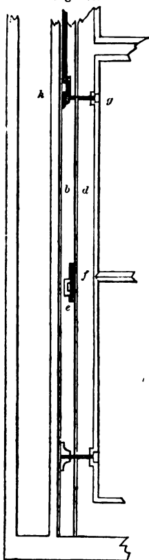
PART ELEVATION OF SHAW'S PATENT WINDOW.
