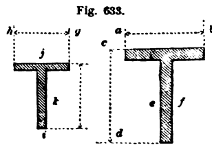
Fig. 633. SECTION OF WROUGHT-IRON RAFTERS.
