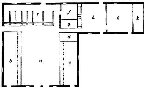
PLAN OF AMERICAN BARN.
