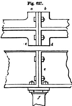
JOINING OF GIRDERS IN THE CAPS OF COLUMNS—SCALE, 1/2 INCH TO THE FOOT.
