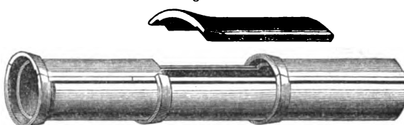
PERSPECTIVE VIEW OF DOULTON'S LIDDED DRAIN-TUBES.
