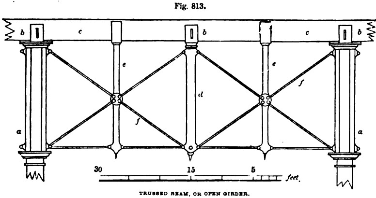
TRUSSED BEAM, OR OPEN GIRDER.
