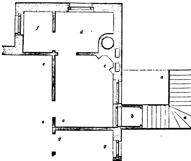
UPPER STOREY OF COMPOSITE COTTAGE APPLIED TO FIG. 75—SCALE IN FIG. 75.
