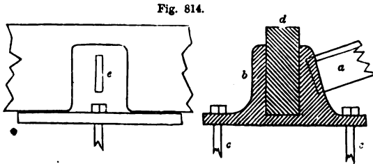
ELEVATION AND SECTION OF SHOE—SCALE, 1 INCH TO THE FOOT.
