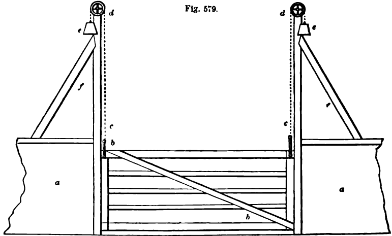
SUSPENDED OR HANGING GATE FOR COURTYARDS—SCALE, 1/4 INCH TO THE FOOT.
