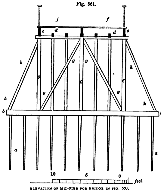
ELEVATION OF MID-PIER FOR BRIDGE IN FIG. 560.
