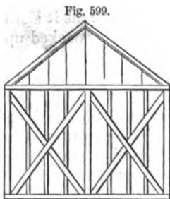
END ELEVATION OF SHED.
