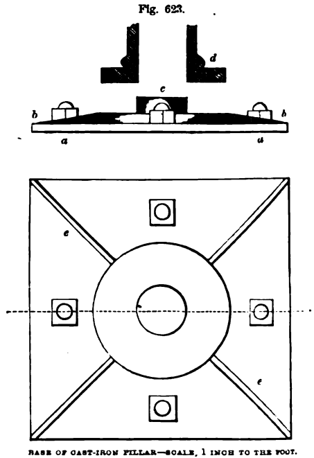
BASE OF CAST-IRON PILLAR—SCALE, 1 INCH TO THE FOOT.
