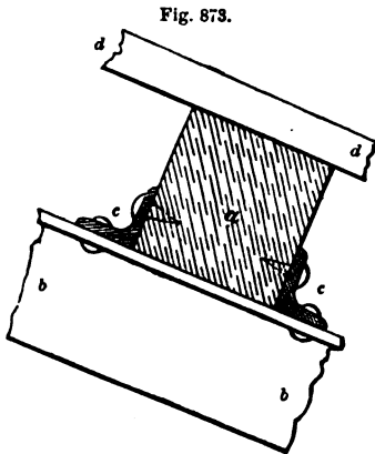
JUNCTION OF WOODEN PURLINS WITH IRON RAFTERS—SCALE IN FIG. 857.
