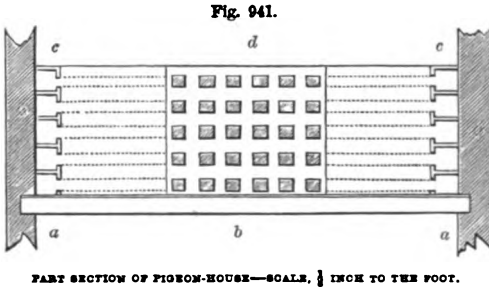
PART SECTION OF PIGEON-HOUSE—SCALE, 1/2 INCH TO THE FOOT.
