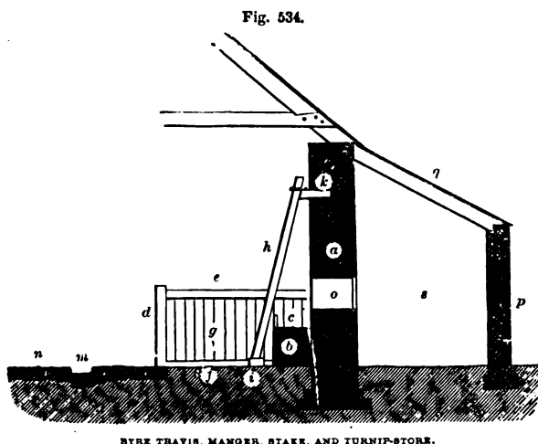
BYRE TRAVIS, MANGER, STAKE, AND TURNIP-STORE.
