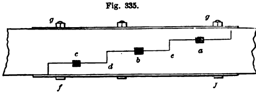
SCARF JOINT—SCALE, 1/4 INCH TO THE FOOT.
