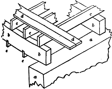
DOUBLE FLOORING—SCALE. 1/4 INCH TO THE FOOT.
