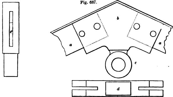
ELEVATIONS AND PLAN OF SHOE FOR UPPER TERMINATION OF RAFTERS—SCALE, 1\frac{1}{2} INCH TO THE FOOT.
