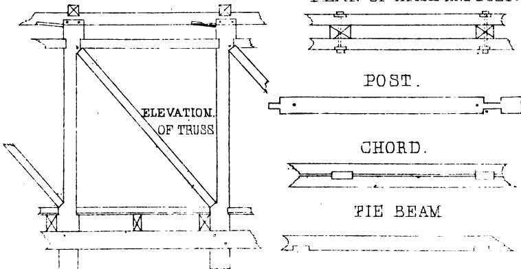
PLAN OF ARCH AND POST.
