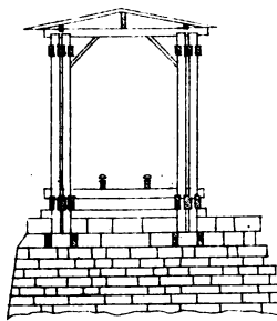
CROSS SECTION.
